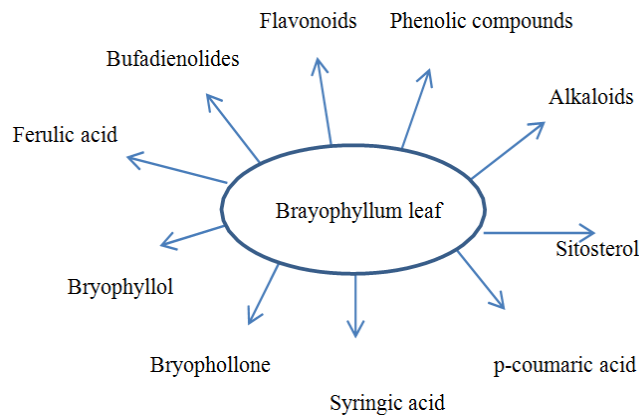
Figure 3: Chemical constituents present in the leaves of Bryophyllum pinnatum .
