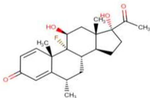
Fig. 1: Structure of Fluorometholone.
